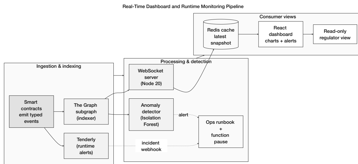
Figure 4.4: Real-time dashboard and runtime monitoring pipeline: smart contracts emit typed events; The Graph indexes them and pushes to a Node WebSocket server which renders the React dashboard via a Redis snapshot. Tenderly runtime alerts and an Isolation-Forest anomaly detector feed the operations runbook with the granular-pause control surface of Section 3.19.
