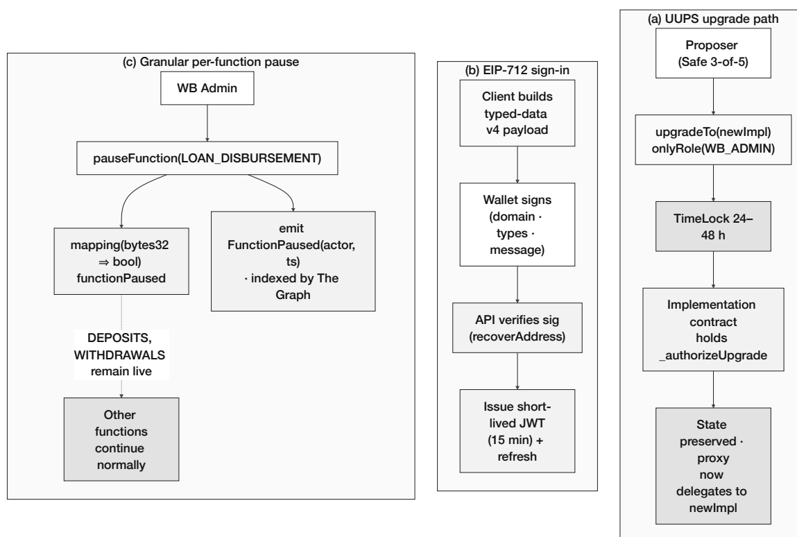
Figure 3.31: Smart-contract security controls: (a) UUPS (ERC-1822) upgrade path with TimeLock-gated authorization; (b) EIP-712 sign-in (typed-data v4 with domain separation and 15-minute JWT); (c) granular per-function pause registry indexed by The Graph for transparent governance.
