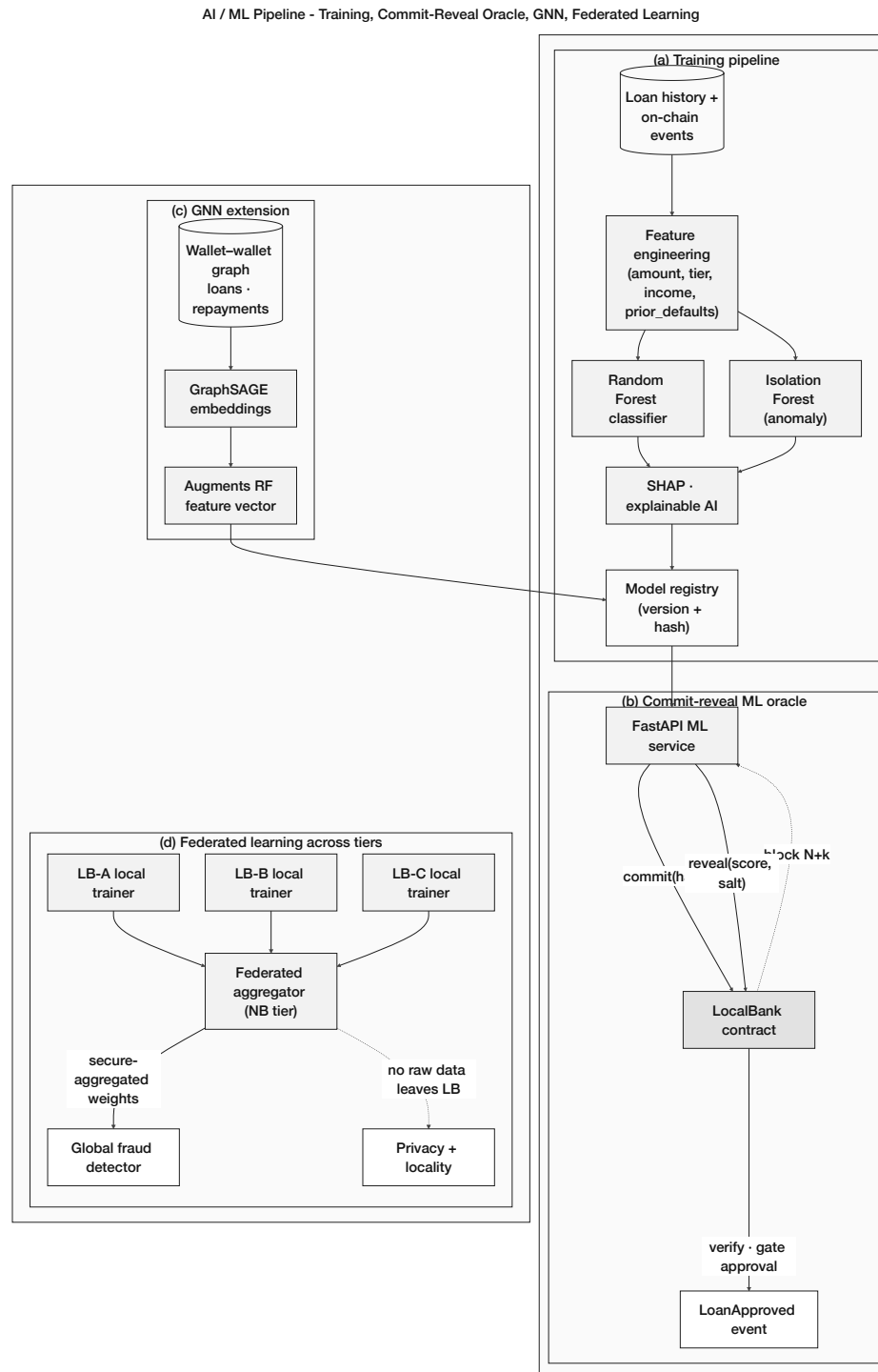
Figure 4.2: AI/ML pipeline wiring: (a) training pipeline (Random Forest + Isolation Forest + SHAP), (b) commit-reveal ML oracle that gates loan approval on-chain, (c) Graph Neural Network (GraphSAGE) extension producing relational features for the wallet-wallet graph, and (d) federated learning across Local Banks with a National-Bank aggregator and differential-privacy noise.
